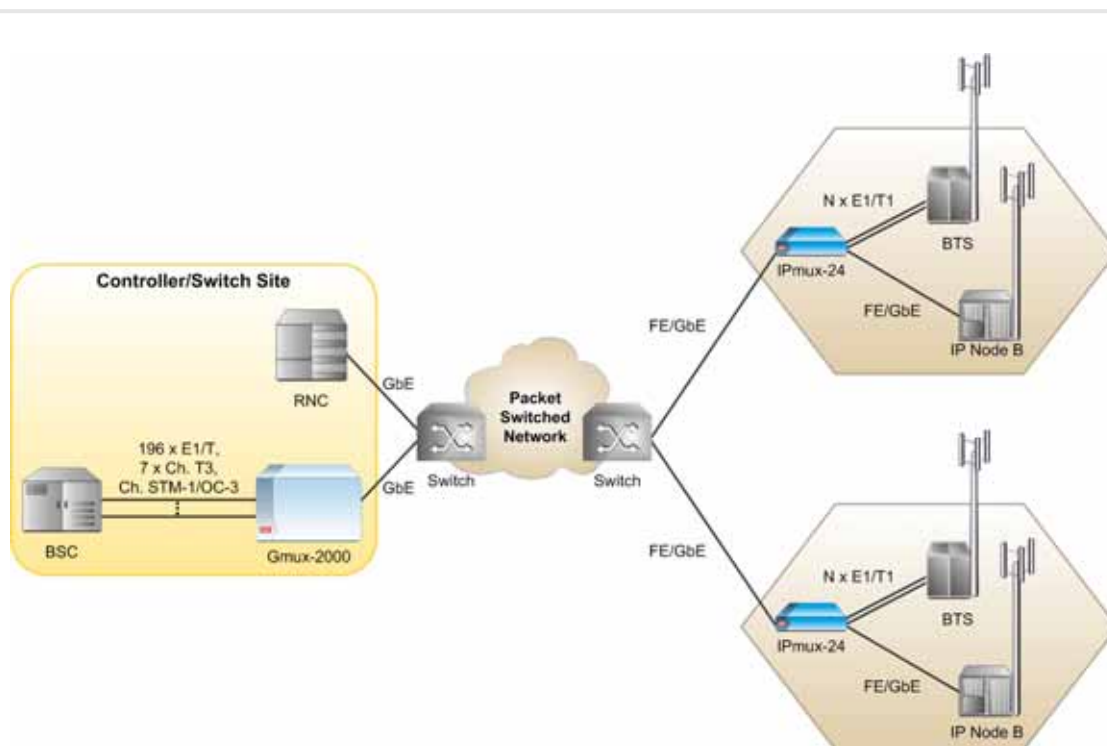
Figure 1. 2G/3G Cellular Backhaul
