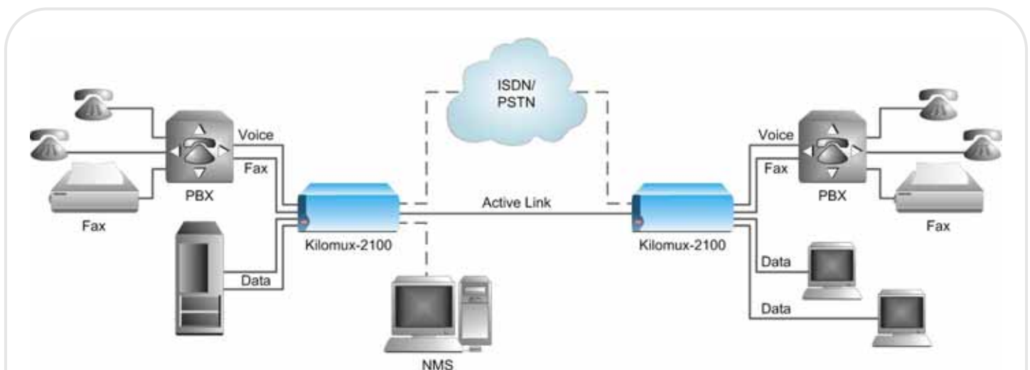
Figure 3. Point-to-point Topology
