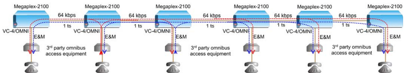
Figure 5. Typical Point-to-Multipoint (Omnibus) Connection
