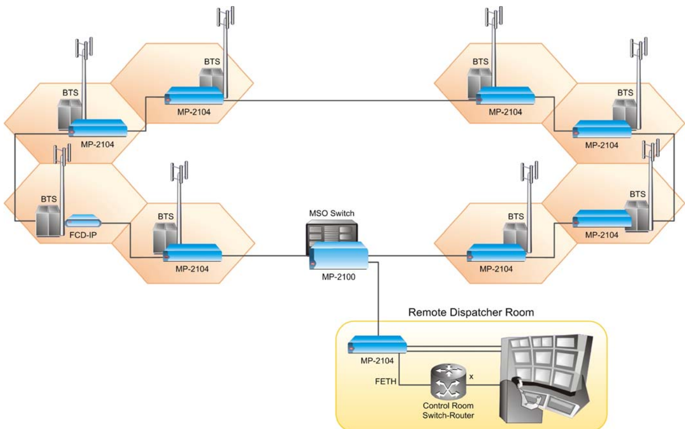
Figure 4. Megaplex-2100 in a Tetra Ring
